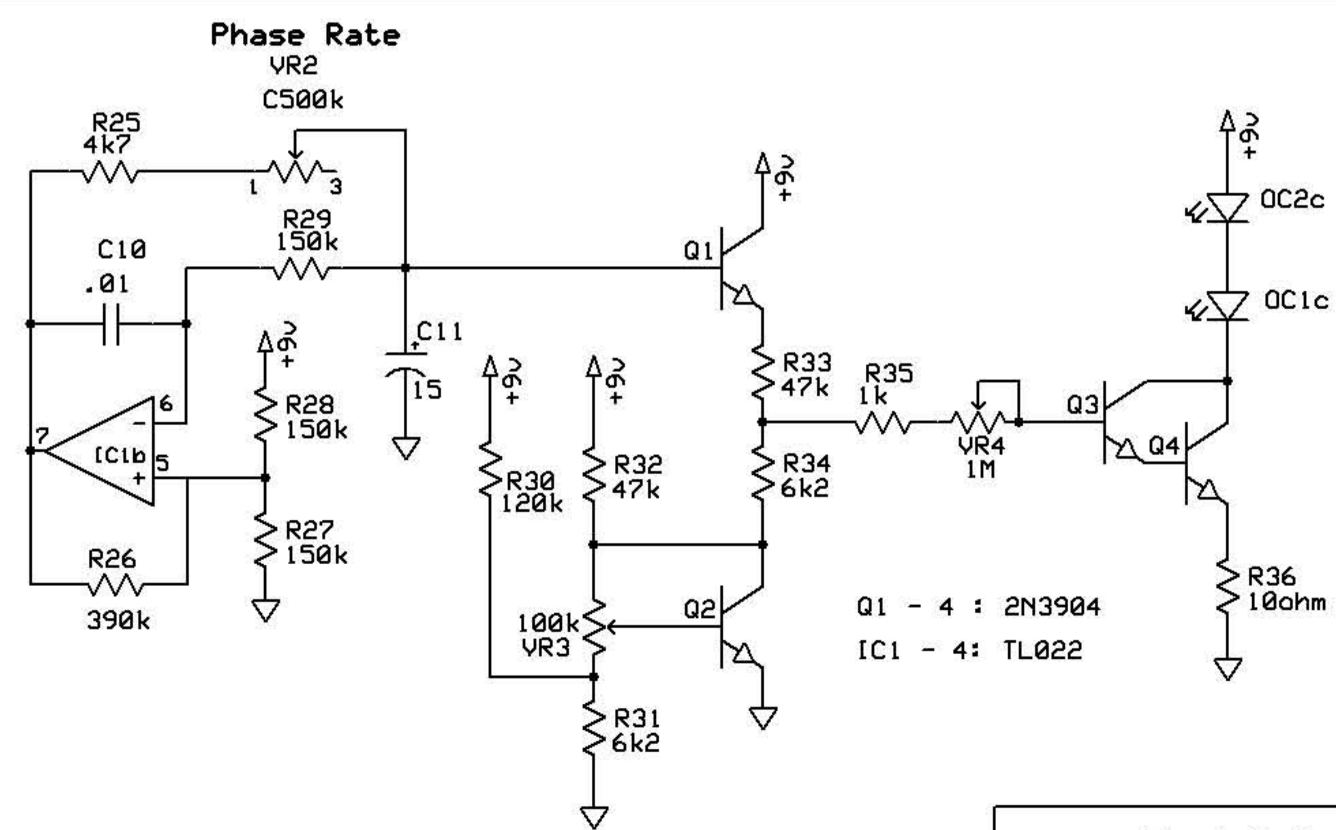
Phaser Circuit
